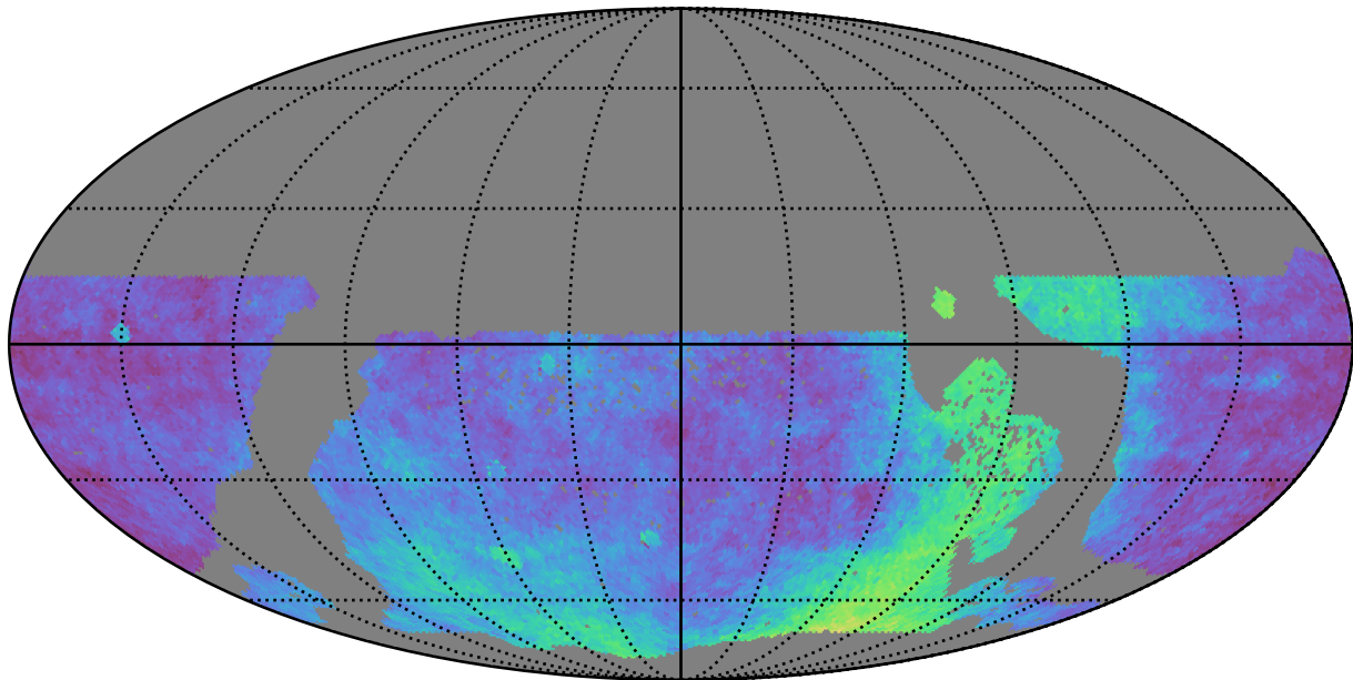
no_magell_roll_v3.4_10yrs WFD: Parallax Coverage @ 22.4
