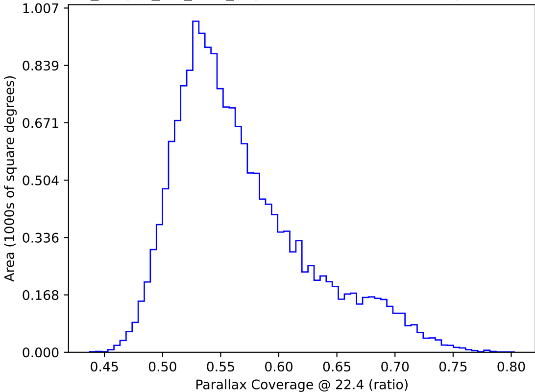
no_magell_roll_v3.4_10yrs WFD: Parallax Coverage @ 22.4
