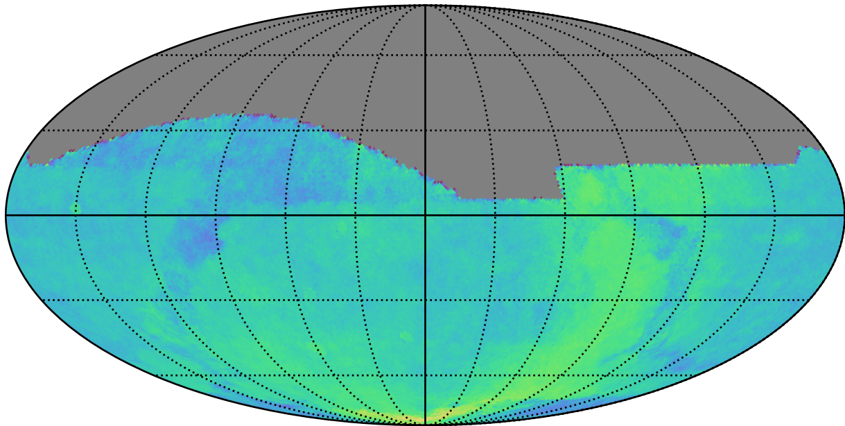
no_magell_roll_v3.4_10yrs All sky: Parallax Coverage @ 22.4
