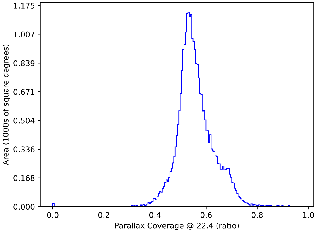
no_magell_roll_v3.4_10yrs All sky: Parallax Coverage @ 22.4
