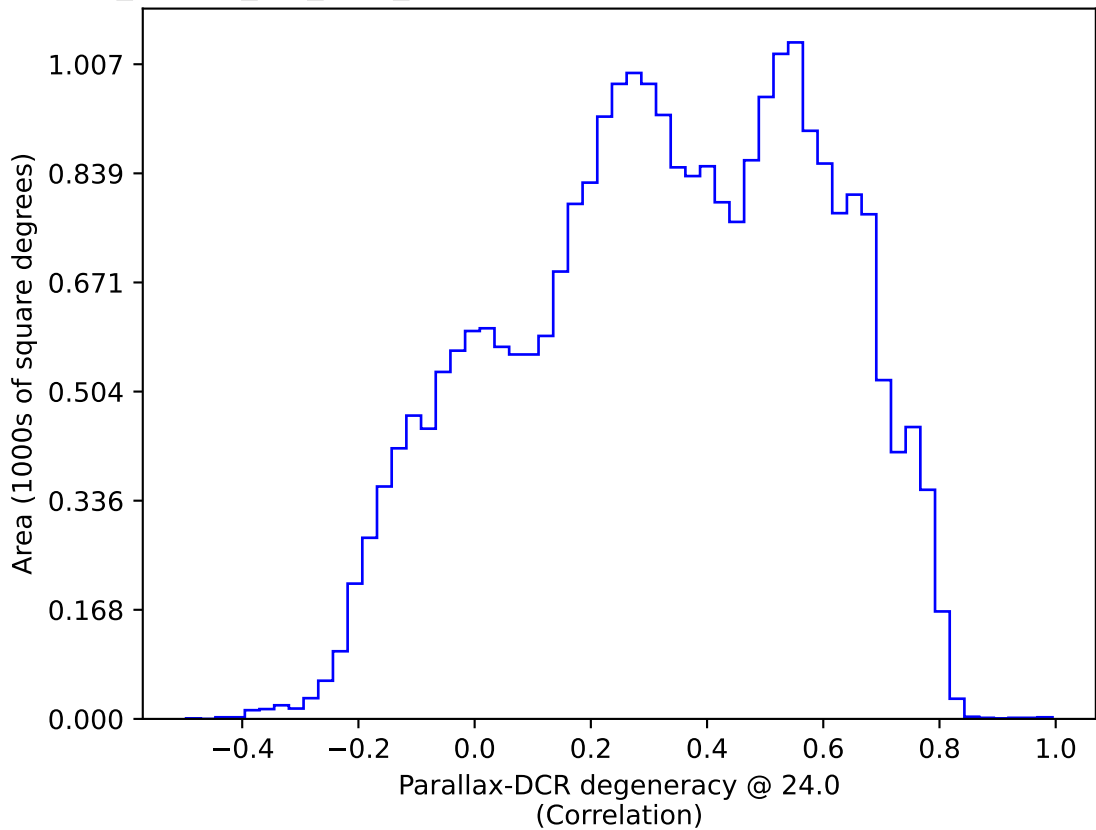
no_magell_roll_v3.4_10yrs All sky: Parallax-DCR degeneracy @ 24.0
