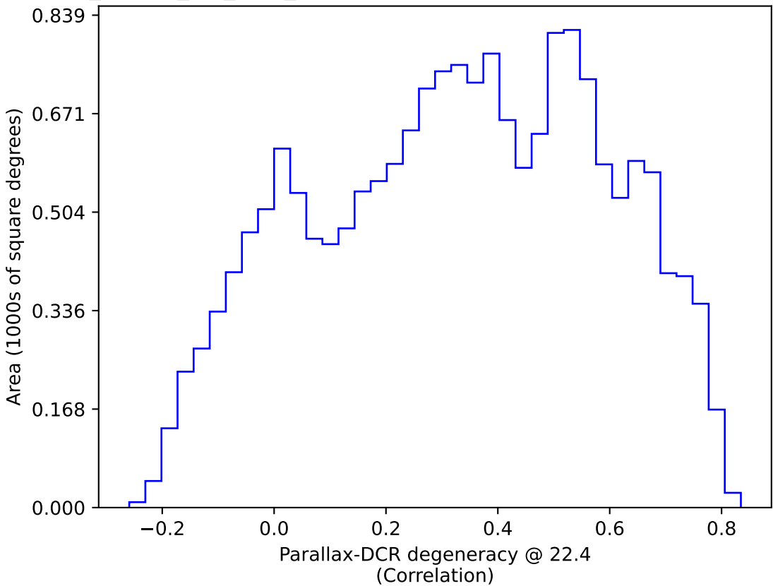
no_magell_roll_v3.4_10yrs WFD: Parallax-DCR degeneracy @ 22.4
