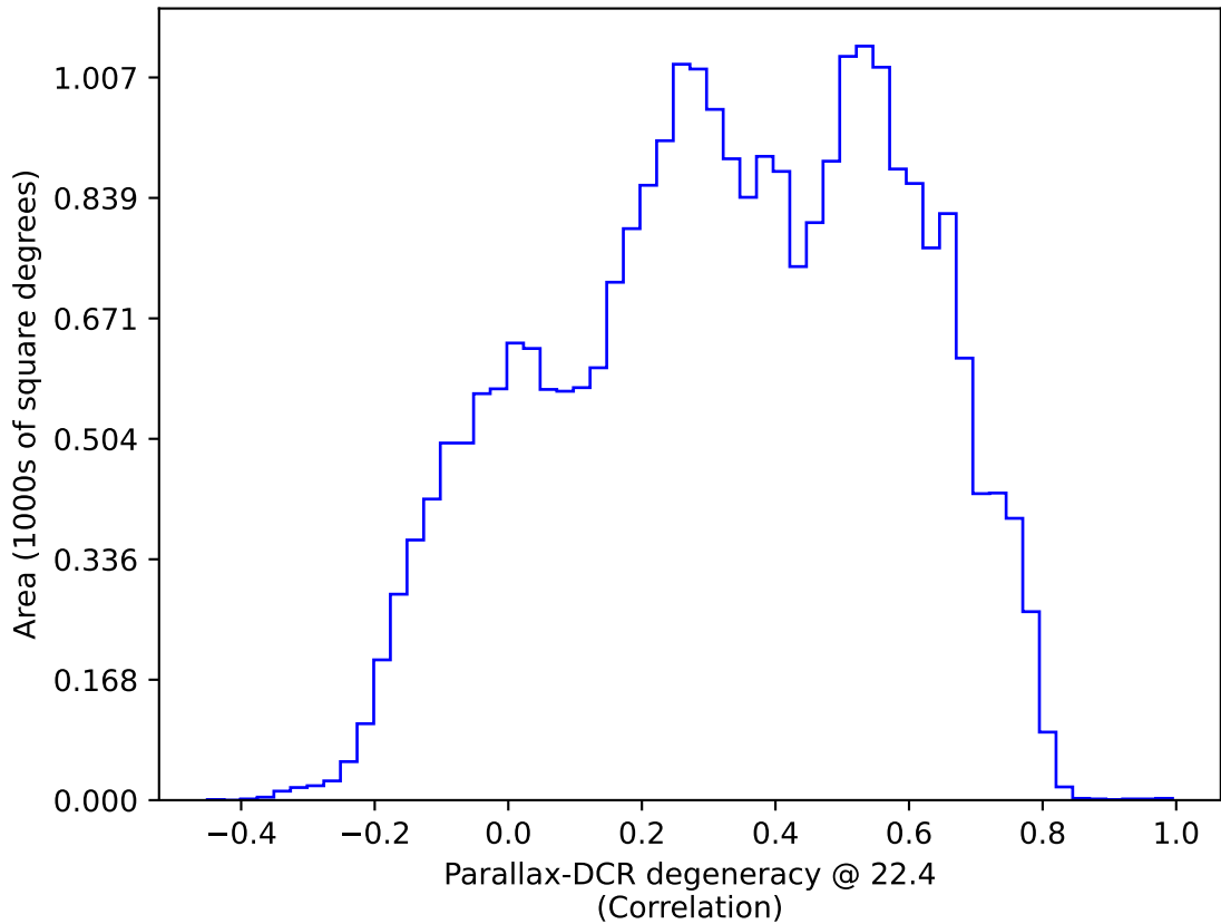
no_magell_roll_v3.4_10yrs All sky: Parallax-DCR degeneracy @ 22.4
