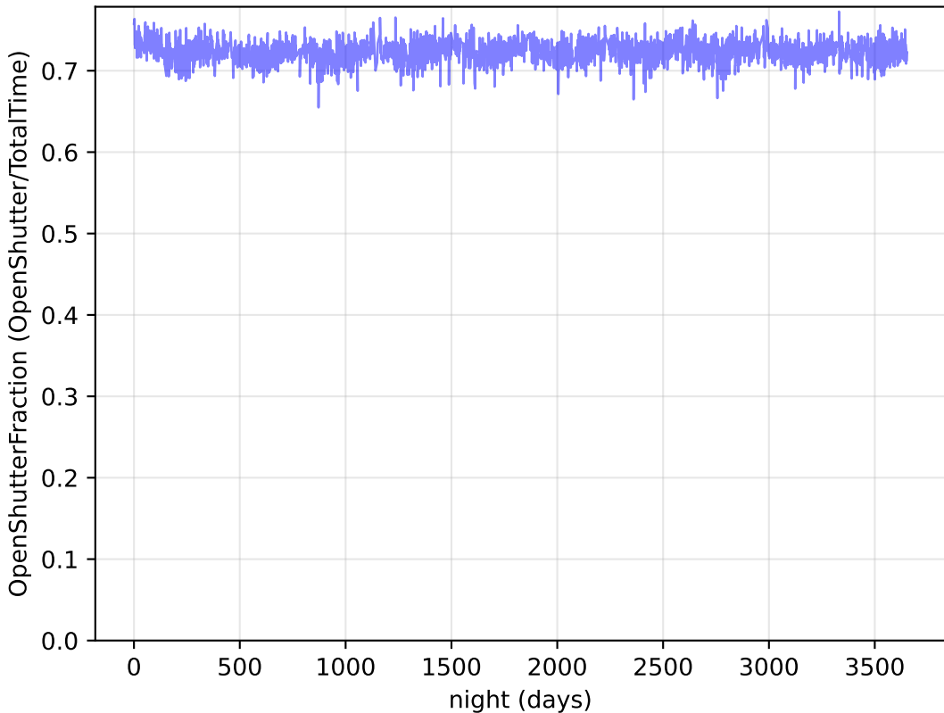
no_magell_roll_v3.4_10yrs Per night: OpenShutterFraction
