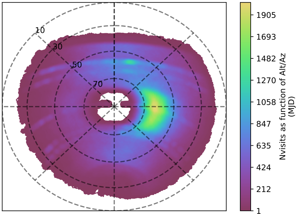
no_magell_roll_v3.4_10yrs y band: Nvisits as function of Alt/Az
