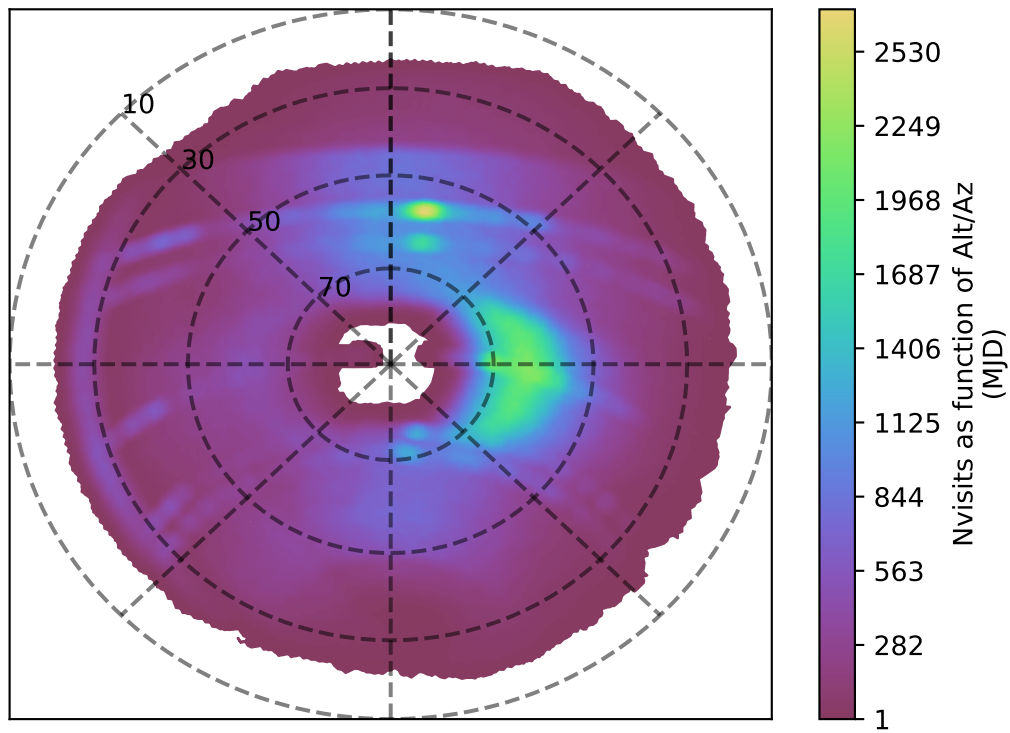
no_magell_roll_v3.4_10yrs r band: Nvisits as function of Alt/Az
