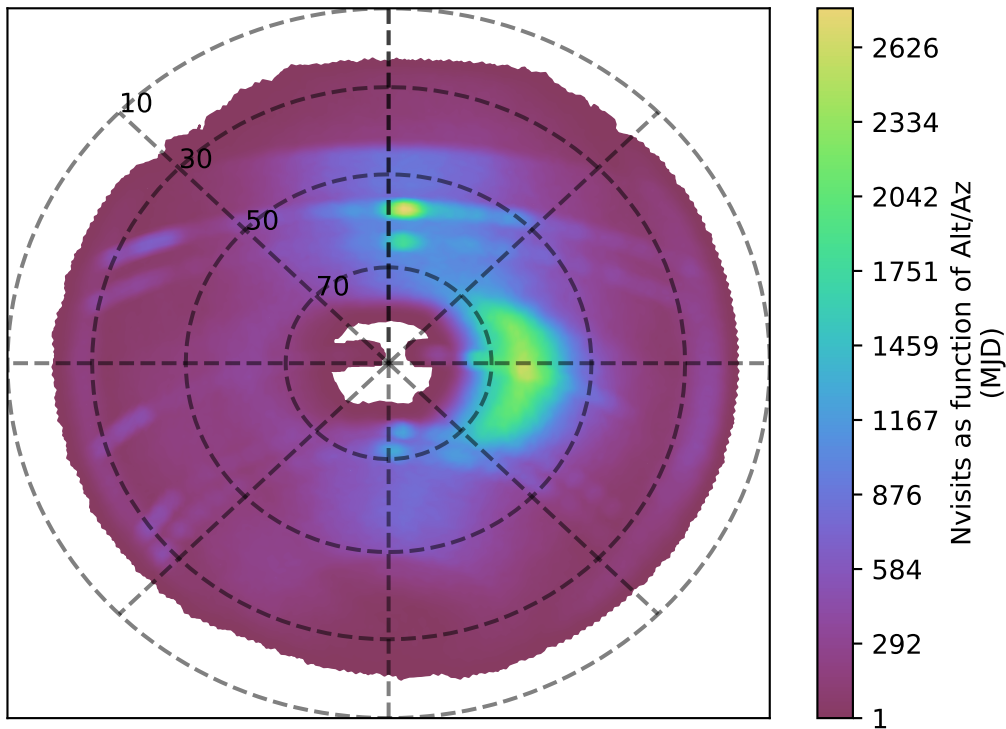
no_magell_roll_v3.4_10yrs i band: Nvisits as function of Alt/Az
