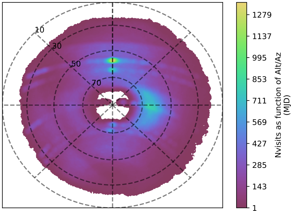
no_magell_roll_v3.4_10yrs g band: Nvisits as function of Alt/Az
