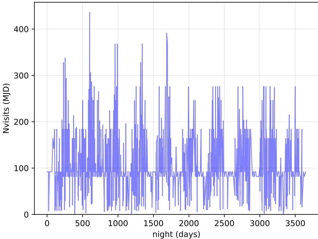
no_magell_roll_v3.4_10yrs DDF: Nvisits
