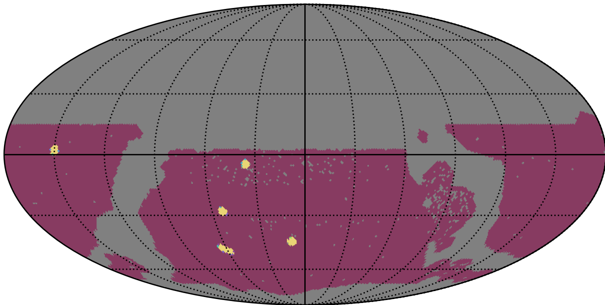
no_magell_roll_v3.4_10yrs WFD: NumberOfQuickRevisits
