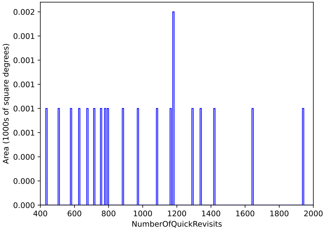
no_magell_roll_v3.4_10yrs WFD: NumberOfQuickRevisits
