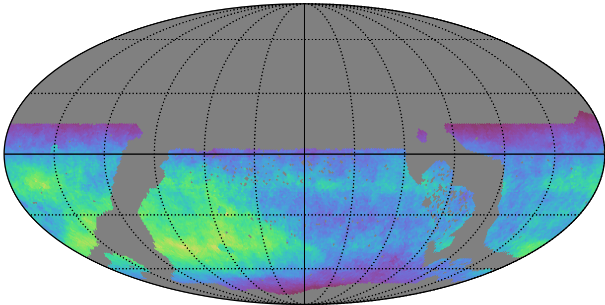
no_magell_roll_v3.4_10yrs WFD z band: Normalized Teff
