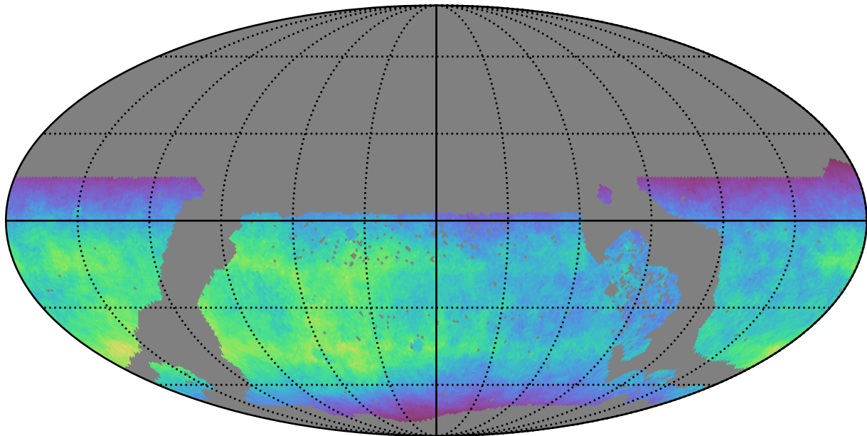
no_magell_roll_v3.4_10yrs WFD y band: Normalized Teff
