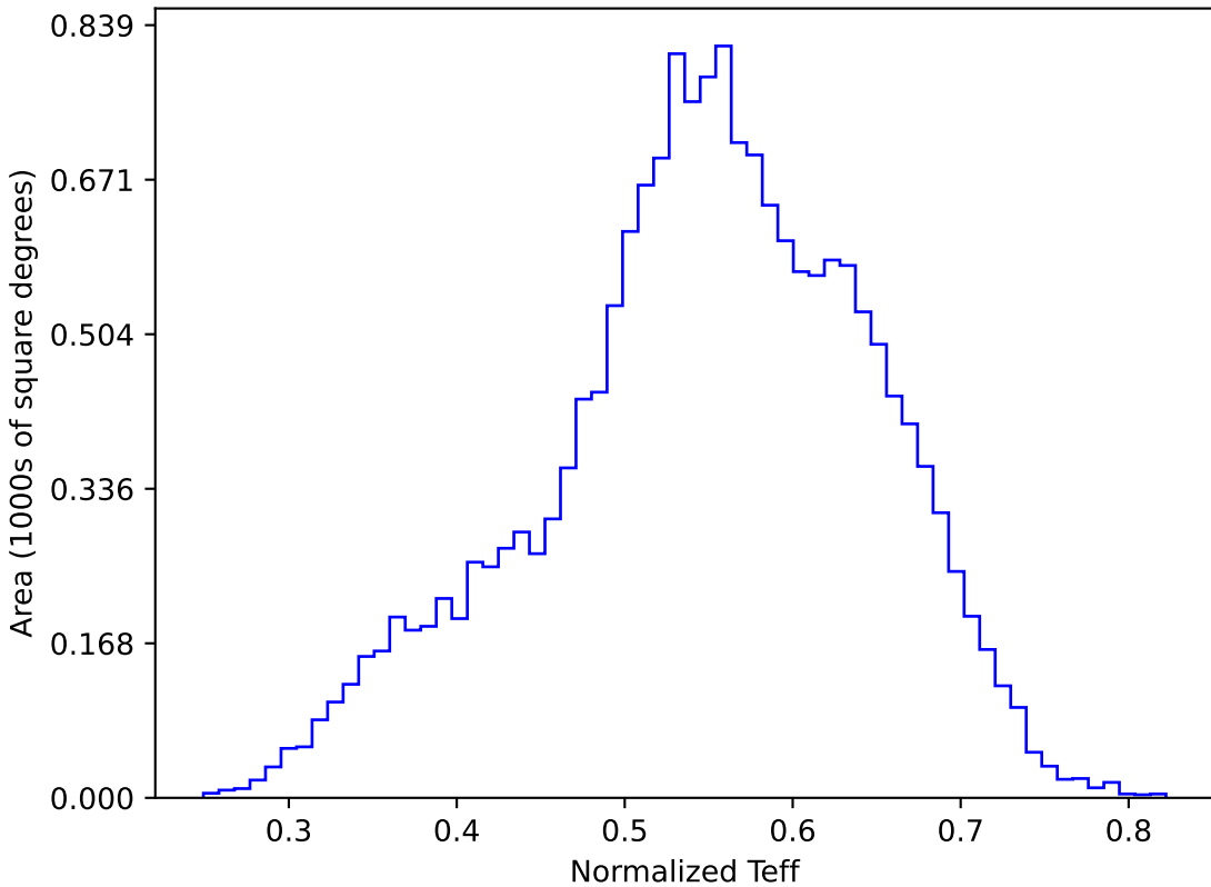
no_magell_roll_v3.4_10yrs WFD y band: Normalized Teff
