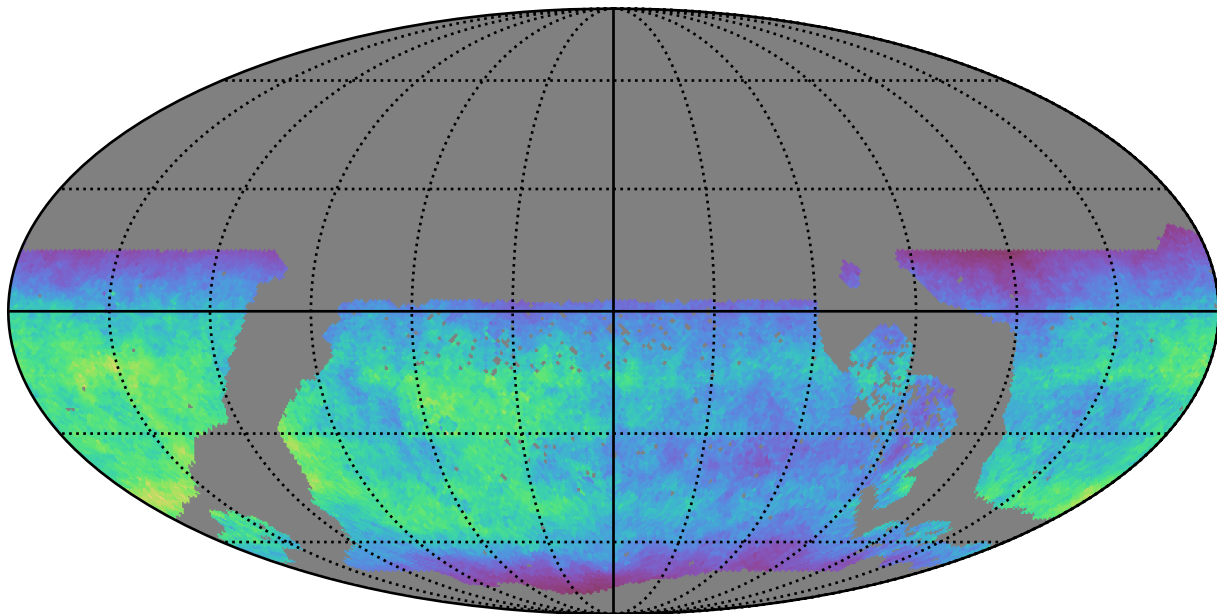
no_magell_roll_v3.4_10yrs WFD u band: Normalized Teff
