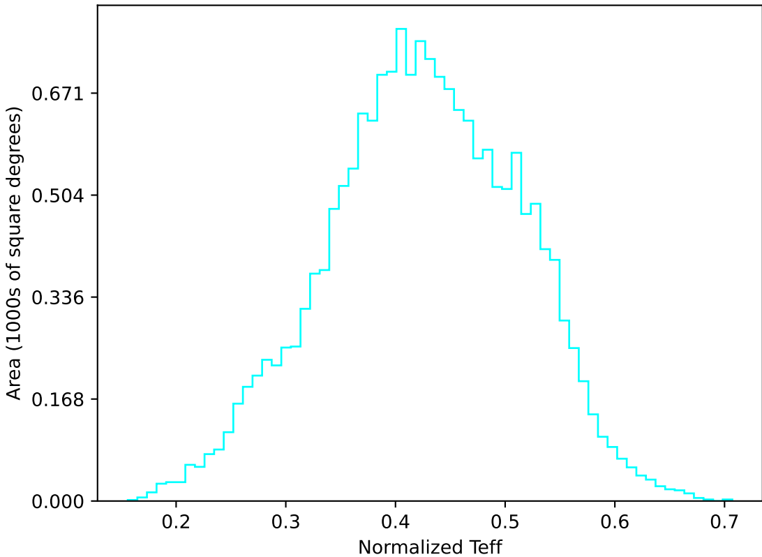
no_magell_roll_v3.4_10yrs WFD u band: Normalized Teff
