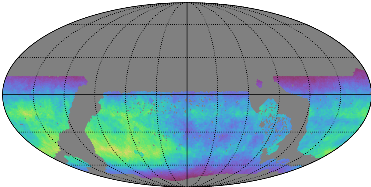
no_magell_roll_v3.4_10yrs WFD i band: Normalized Teff
