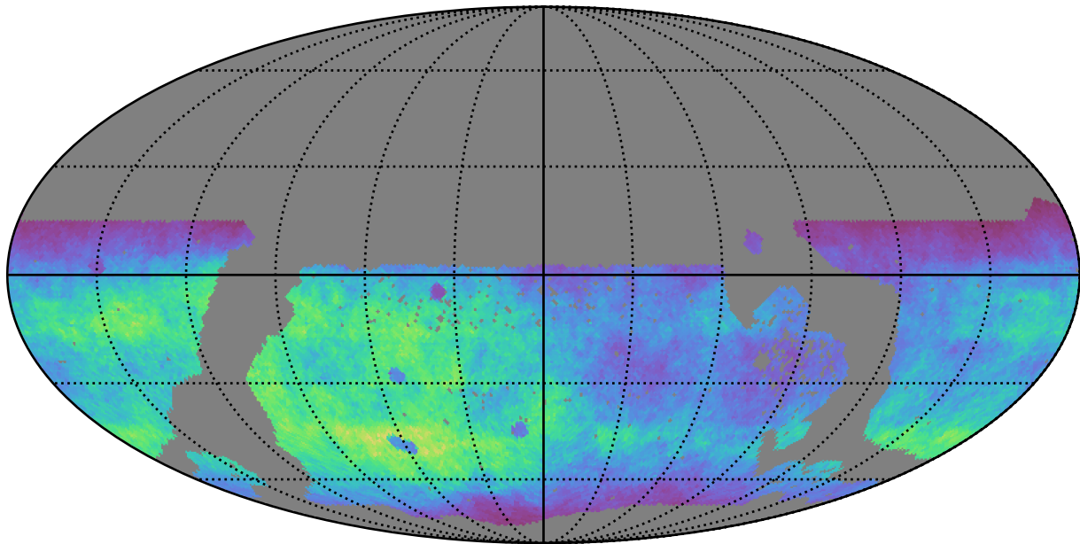
no_magell_roll_v3.4_10yrs WFD g band: Normalized Teff
