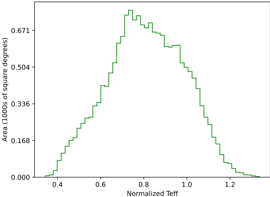
no_magell_roll_v3.4_10yrs WFD g band: Normalized Teff
