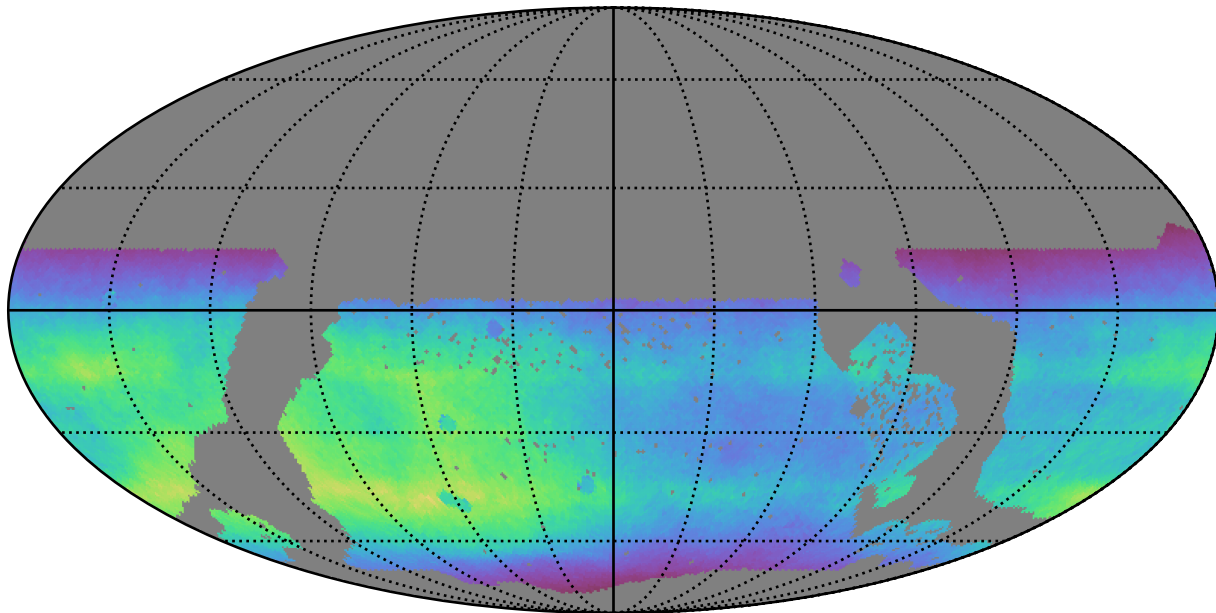
no_magell_roll_v3.4_10yrs WFD all bands: Normalized Teff
