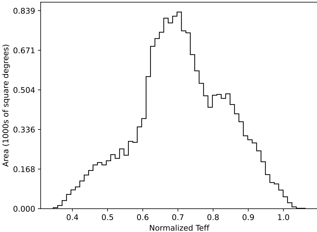
no_magell_roll_v3.4_10yrs WFD all bands: Normalized Teff
