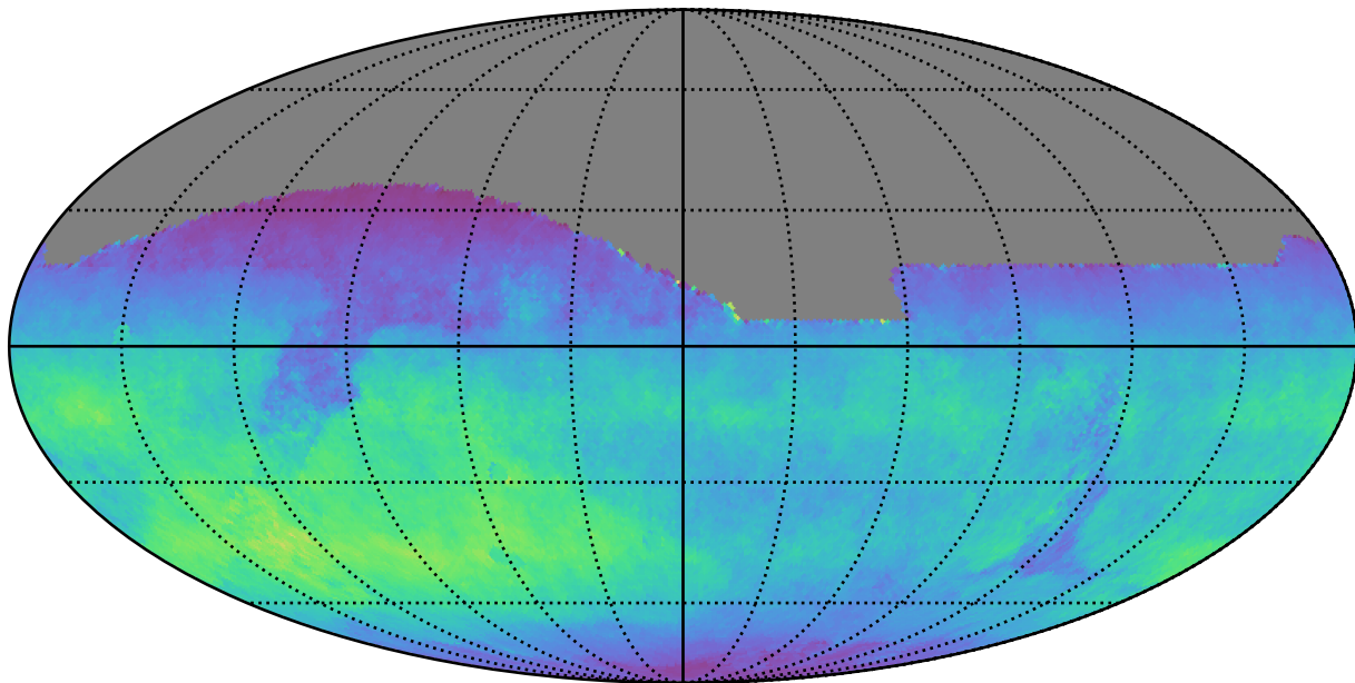
no_magell_roll_v3.4_10yrs All sky z band: Normalized Teff
