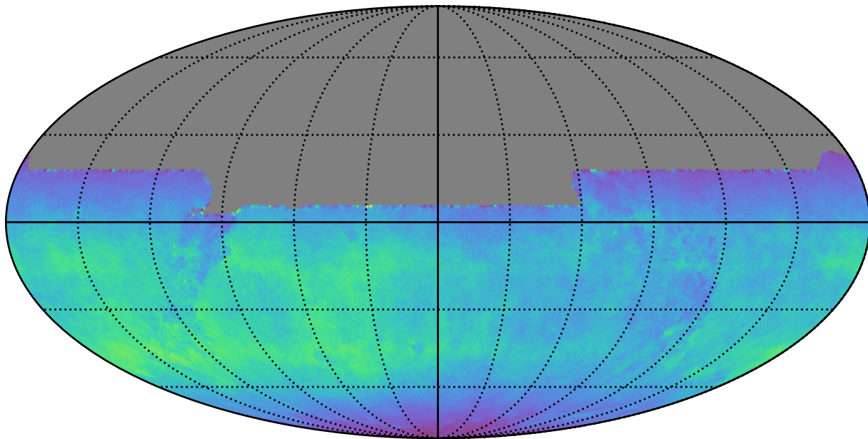
no_magell_roll_v3.4_10yrs All sky y band: Normalized Teff
