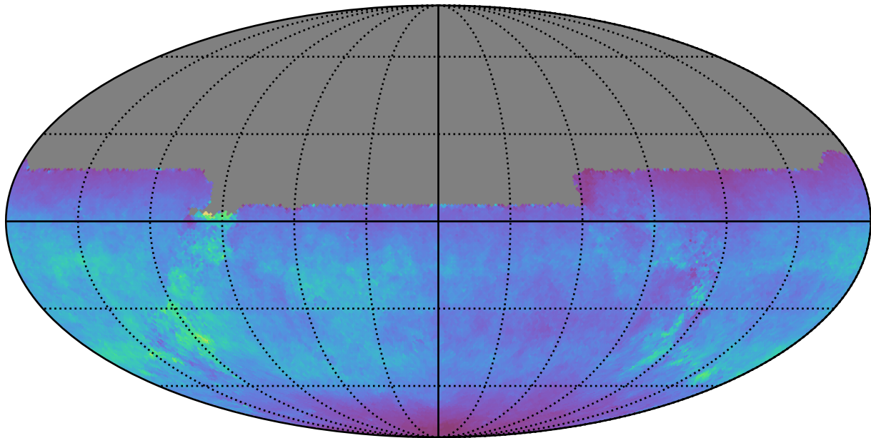
no_magell_roll_v3.4_10yrs All sky u band: Normalized Teff
