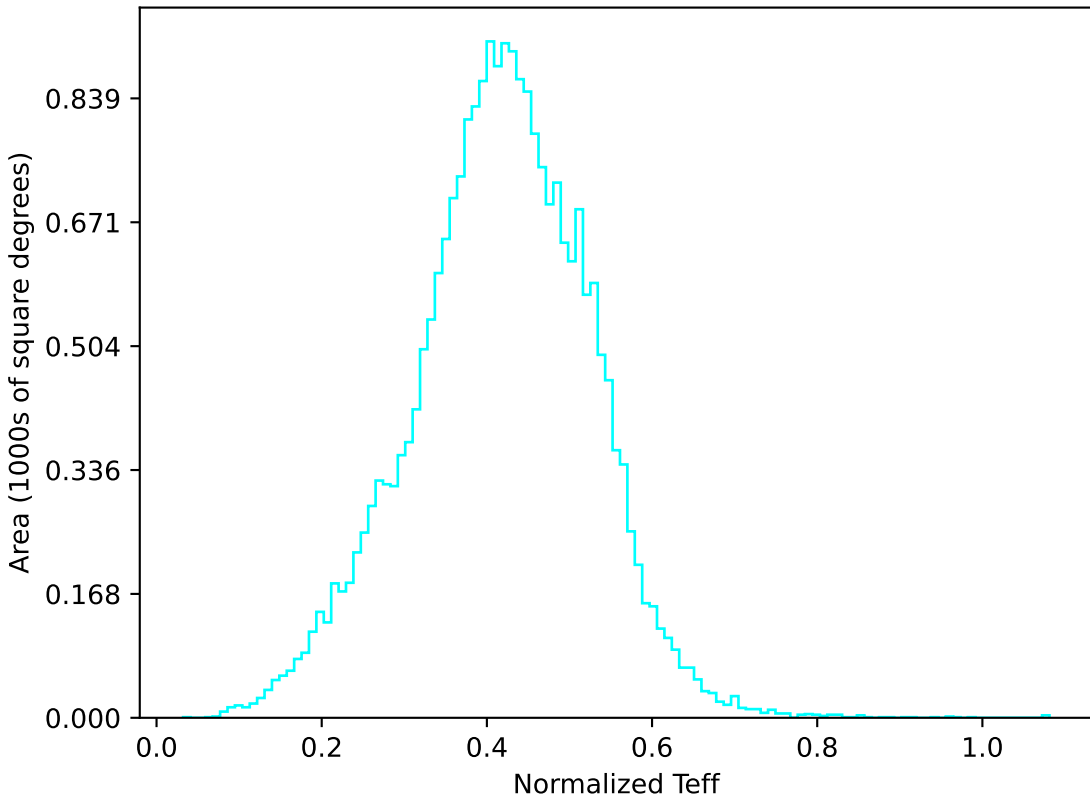
no_magell_roll_v3.4_10yrs All sky u band: Normalized Teff
