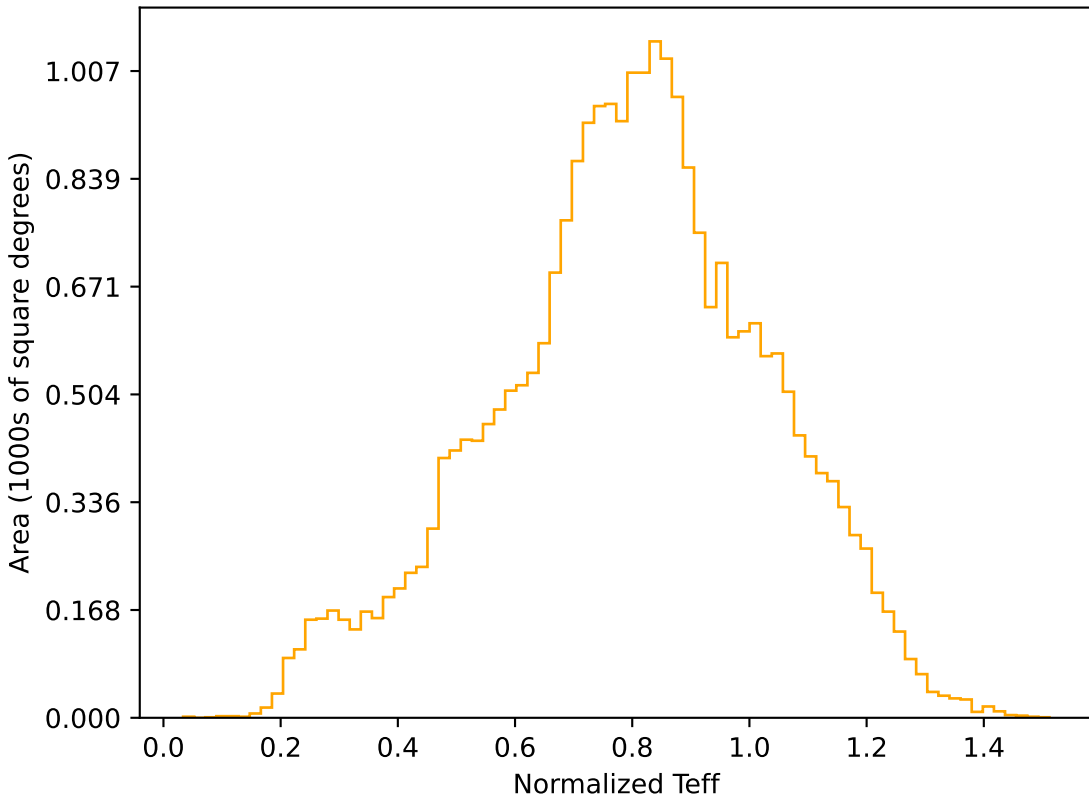
no_magell_roll_v3.4_10yrs All sky r band: Normalized Teff
