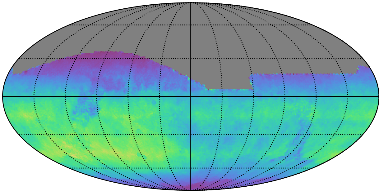
no_magell_roll_v3.4_10yrs All sky i band: Normalized Teff
