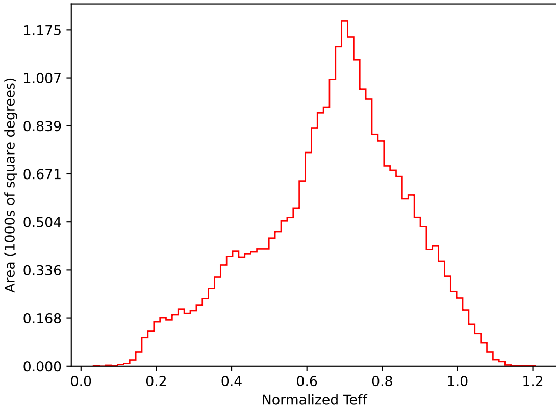
no_magell_roll_v3.4_10yrs All sky i band: Normalized Teff
