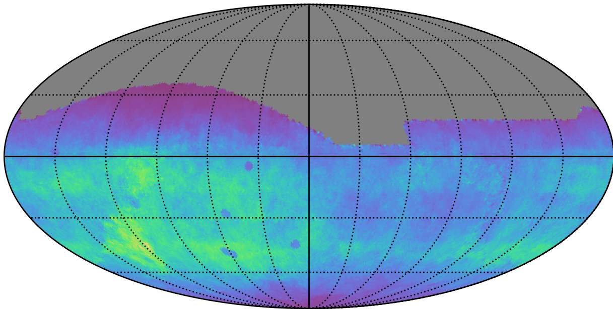
no_magell_roll_v3.4_10yrs All sky g band: Normalized Teff
