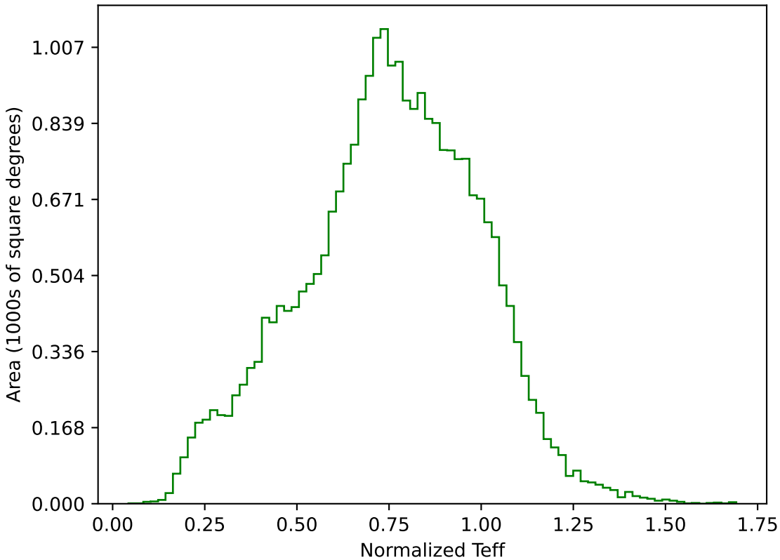
no_magell_roll_v3.4_10yrs All sky g band: Normalized Teff
