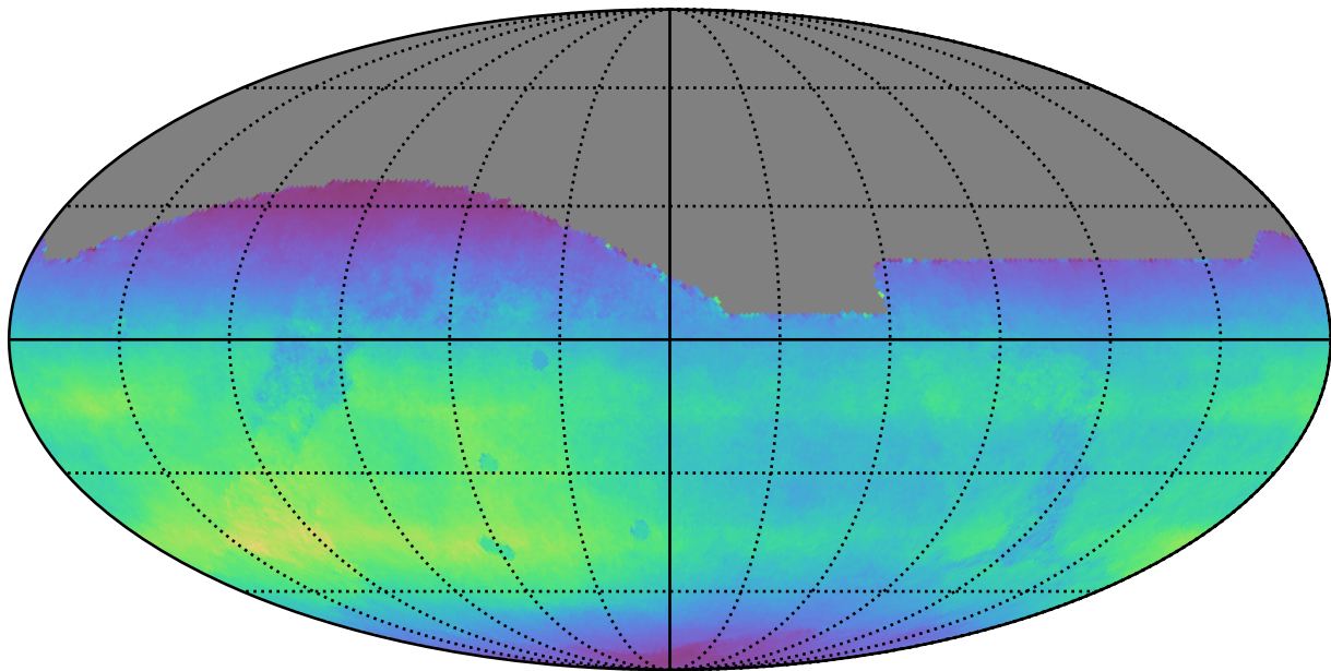
no_magell_roll_v3.4_10yrs All sky all bands: Normalized Teff
