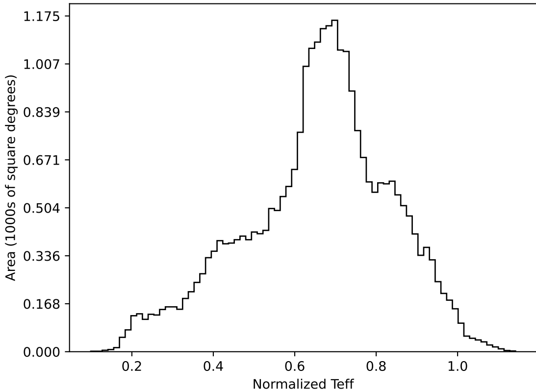
no_magell_roll_v3.4_10yrs All sky all bands: Normalized Teff
