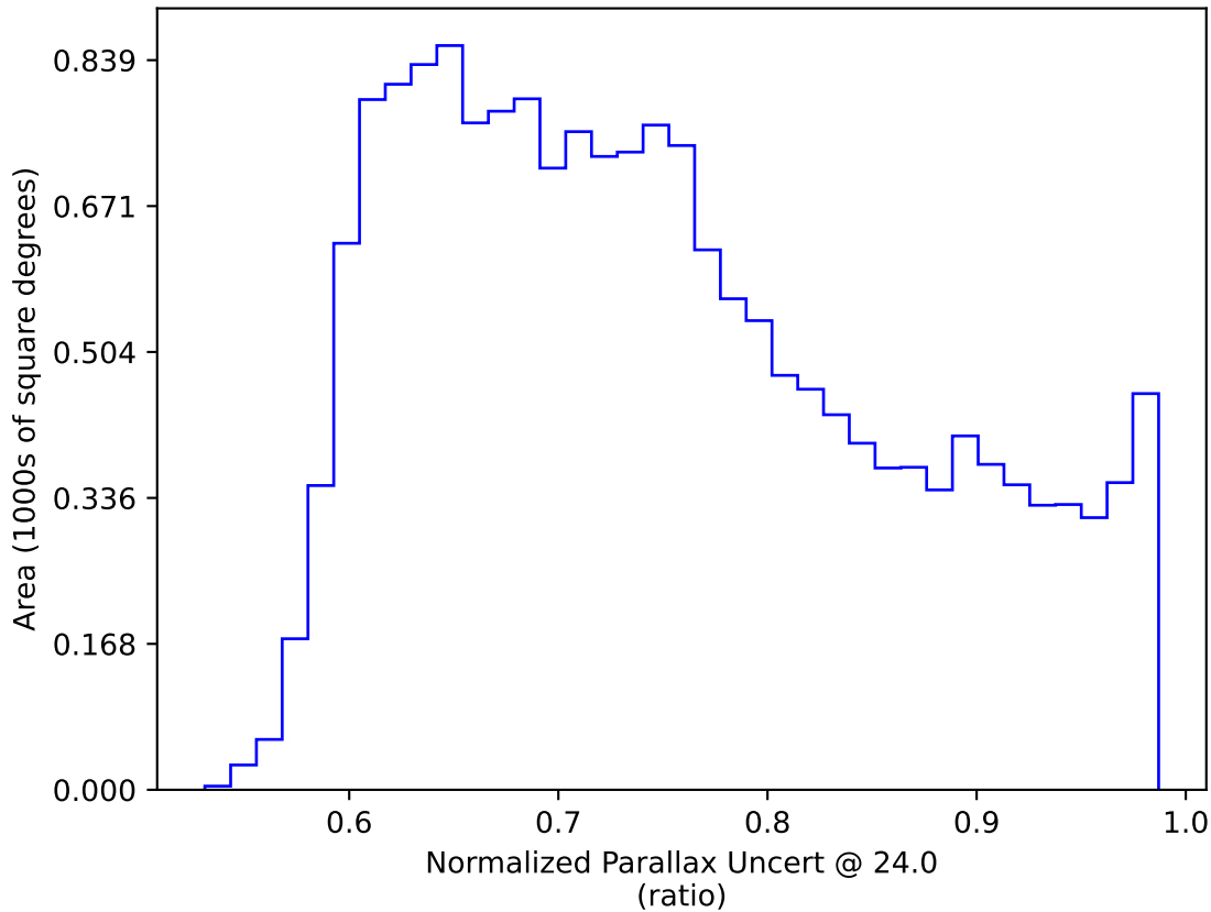
no_magell_roll_v3.4_10yrs WFD: Normalized Parallax Uncert @ 24.0
