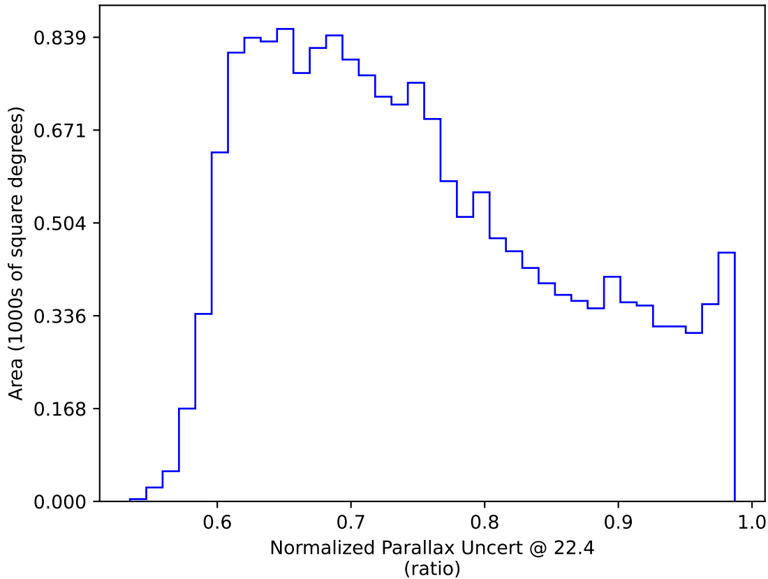
no_magell_roll_v3.4_10yrs WFD: Normalized Parallax Uncert @ 22.4
