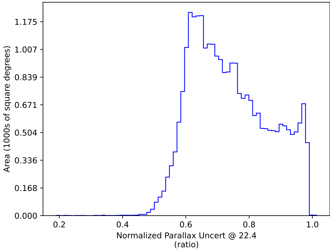
no_magell_roll_v3.4_10yrs All sky: Normalized Parallax Uncert @ 22.4
