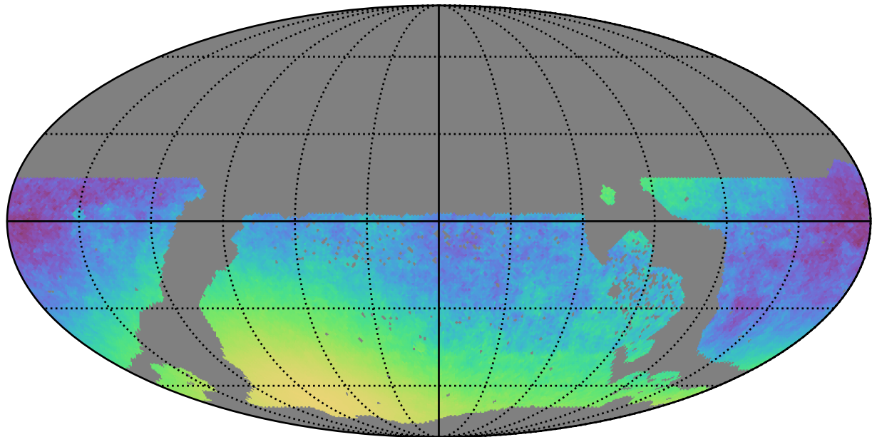
no_magell_roll_v3.4_10yrs WFD y band only: Normalized Parallax Uncert @ 21.3
