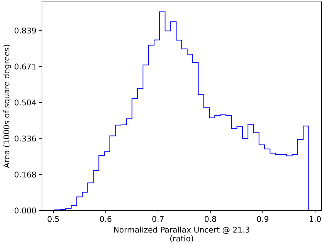
no_magell_roll_v3.4_10yrs WFD y band only: Normalized Parallax Uncert @ 21.3
