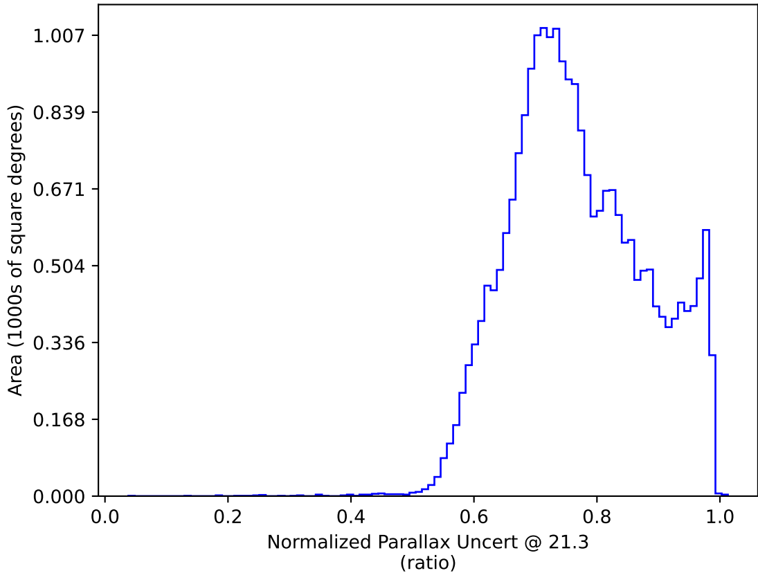
no_magell_roll_v3.4_10yrs All sky y band only: Normalized Parallax Uncert @ 21.3
