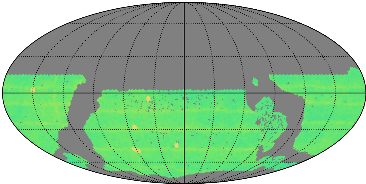
no_magell_roll_v3.4_10yrs WFD all bands: N Unique Nights
