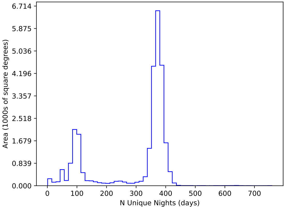
no_magell_roll_v3.4_10yrs All sky all bands: N Unique Nights
