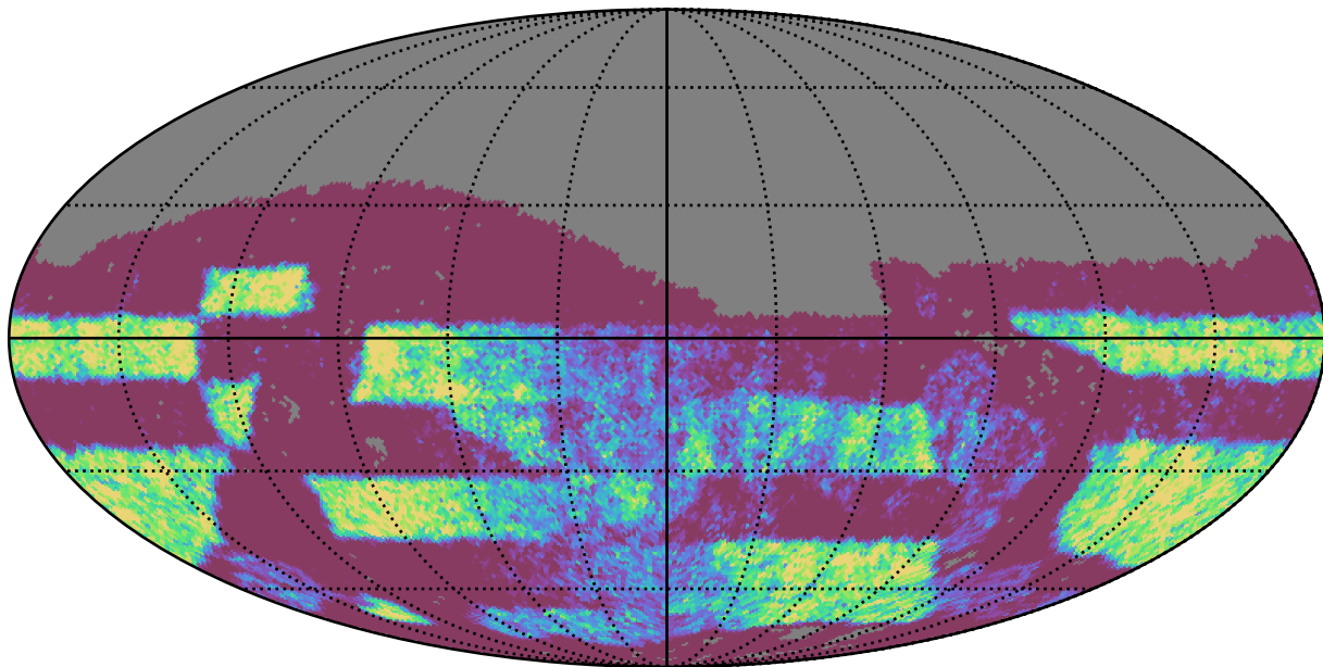
no_magell_roll_v3.4_10yrs Yr 3-4 z band: NVisits
