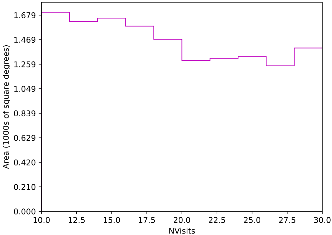
no_magell_roll_v3.4_10yrs Yr 3-4 z band: NVisits
