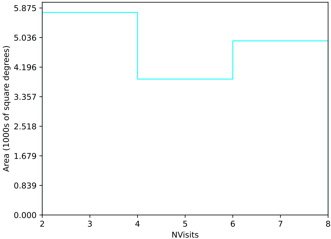
no_magell_roll_v3.4_10yrs Yr 3-4 u band: NVisits
