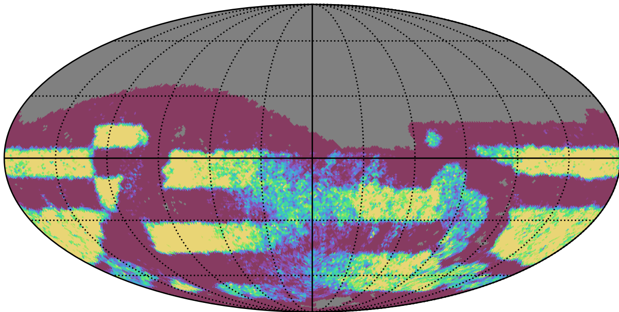
no_magell_roll_v3.4_10yrs Yr 3-4 r band: NVisits
