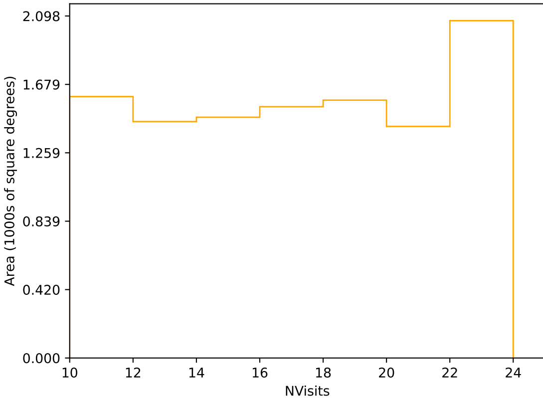
no_magell_roll_v3.4_10yrs Yr 3-4 r band: NVisits
