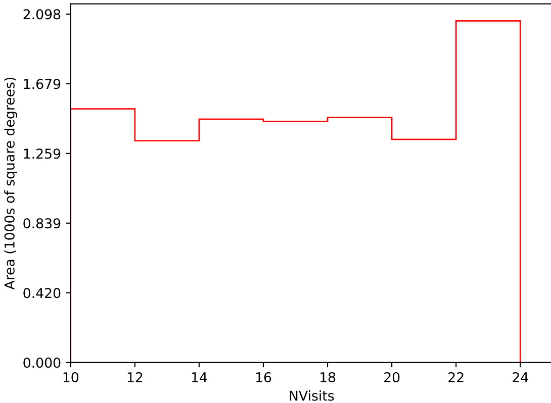
no_magell_roll_v3.4_10yrs Yr 3-4 i band: NVisits
